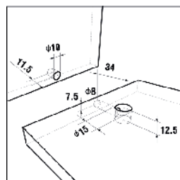
Conector minifix
